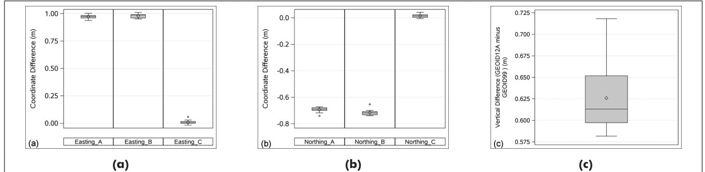
Figure 14. Boxplots of, (a) easting, and (b) northing differences (in meters) in NAD 83(2011) minus NAD 83(CORS96) for datasets 'A', 'B', and 'C'; and (c) vertical difference (in meters) for GEOID12A minus GEOID99.
