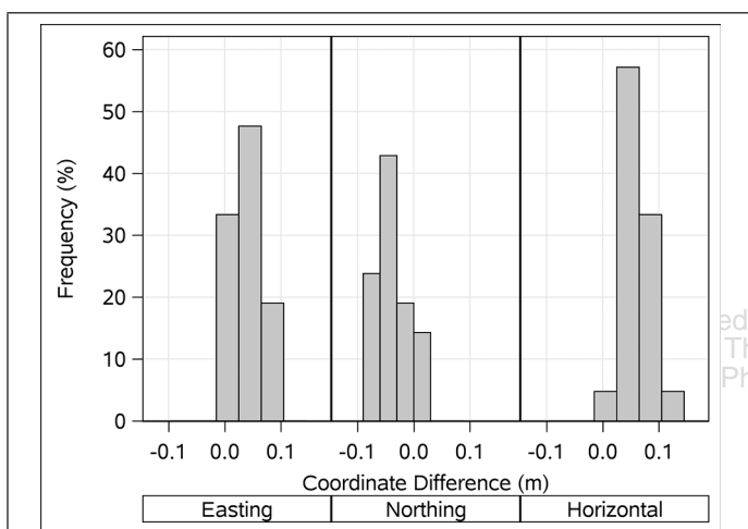
Figure 9. Histogram plots for the differences (m) in easting, northing, and total horizontal Cartesian differences between NAD 83(1986) and NAD 83(NSRS2007).
