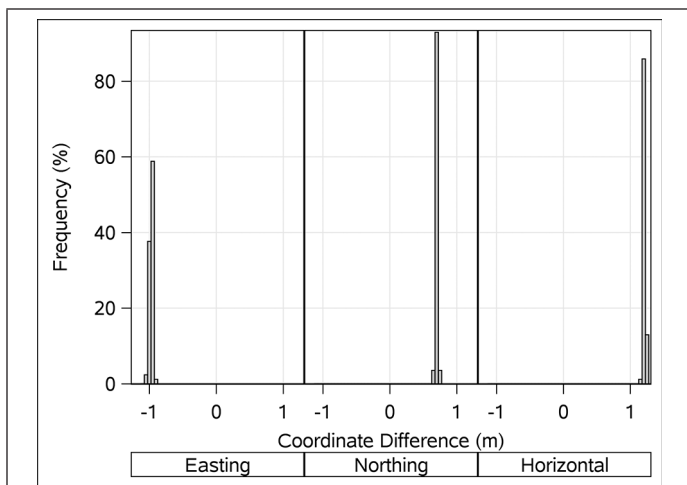
Figure 8. Histogram plots for the difference (m) in easting, northing, and total horizontal Cartesian differences between NAD 83(1986) and NAD 83(2011).
