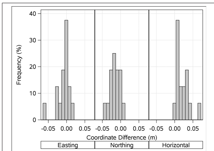
Figure 10. Histogram plots for differences (in meters) in northing and easting, and total horizontal Cartesian distance between NAD 83(CORS96) and NAD 83(2011).
