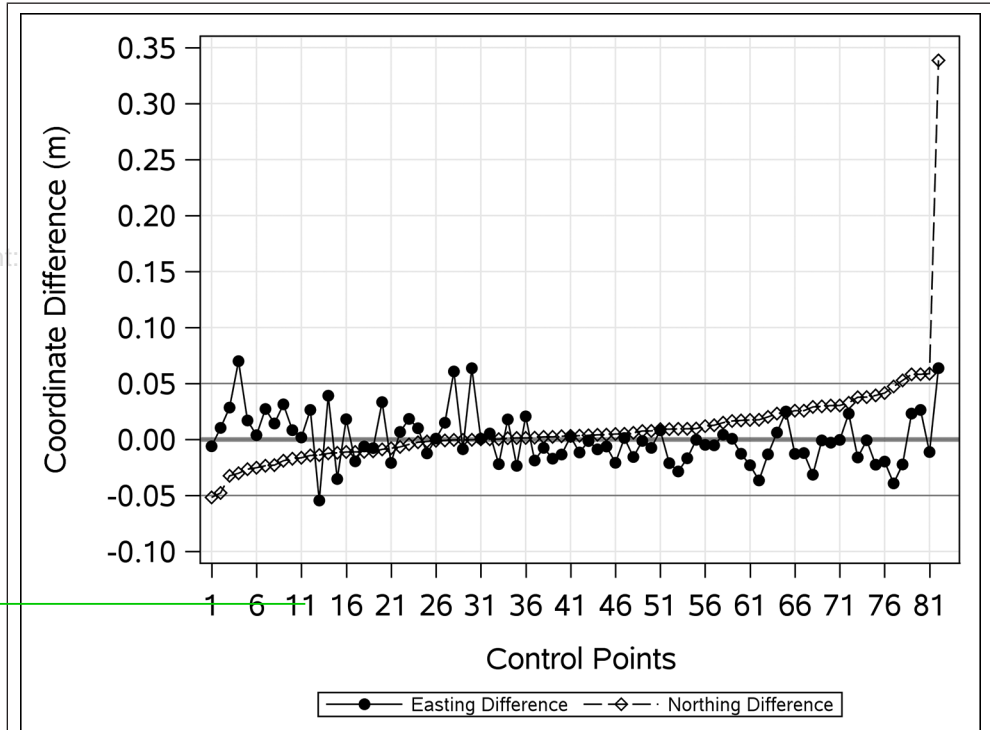
Figure 2. Differences in northing and easting between 2013 and 2015 control point observations using NAD 83(1986).
