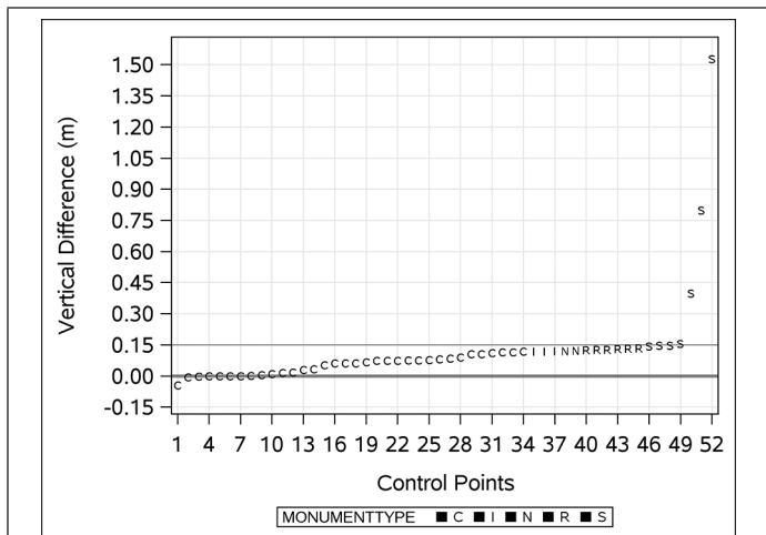
Figure 5. Vertical difference (2013 minus 2015) derived from GEOID03 plotted by the types of monument setting, cement (c), iron (i), nail (n), rebar (r), and stone (s).
