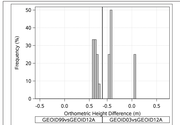
Figure 11. Histogram plots for the differences in orthometric heights (in meters) for GEOID99 versus GEOID12A and GEOID03 versus GEOID12A.
